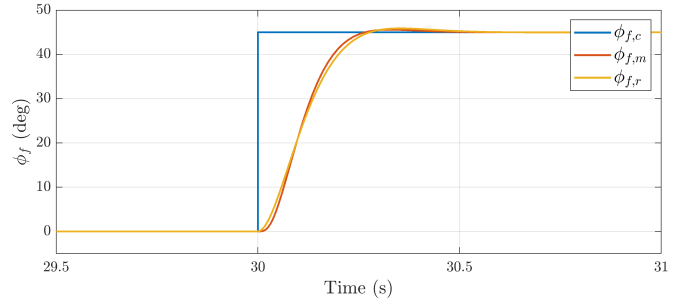
Fig. 2. Closed-loop roll angle step response.
