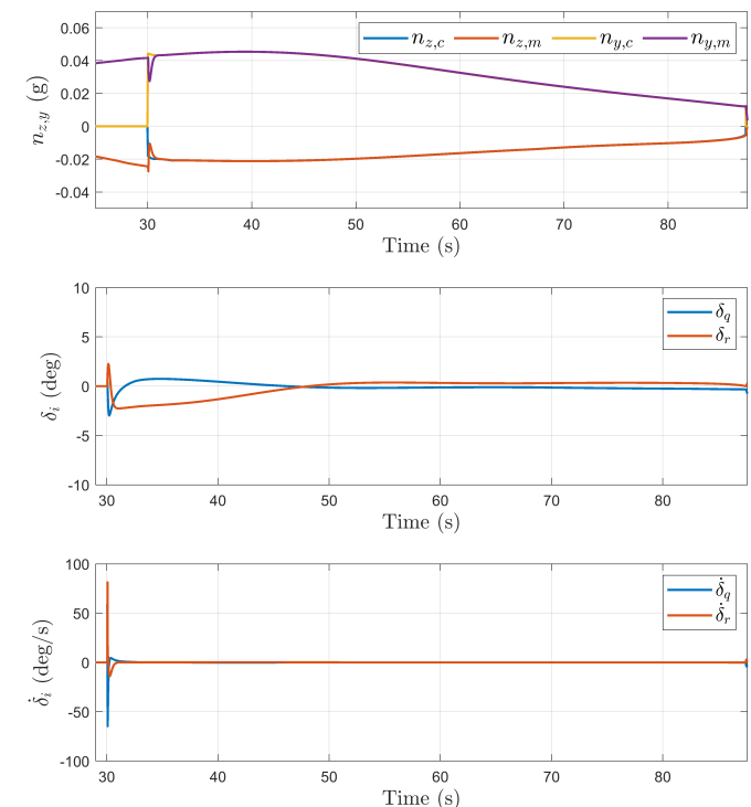
Fig. 8. Nominal simulations: (a) pitch/yaw load factors, (b) deflection angles, (c) deflection angle rates.
