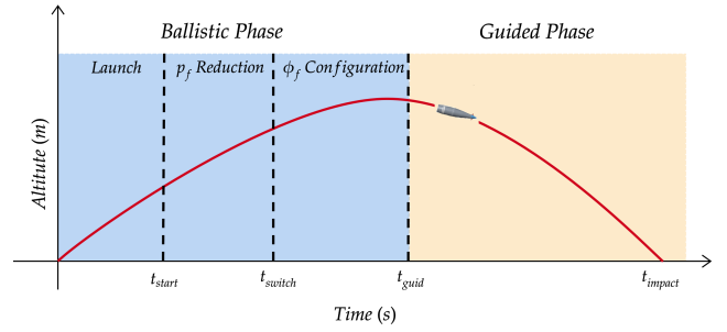
Fig. 6. Projectile flight trajectory.
