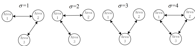
Fig. 1. Switching topologies in a three-area network
