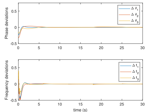
Fig. 3. Phase and frequency deviation for all 3 areas
