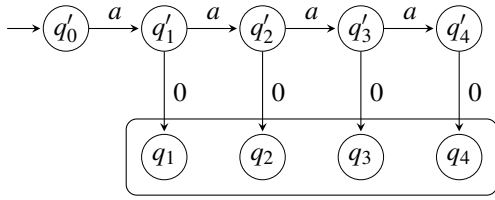
Fig. 3. Construction of an automaton with a single initial state from an automaton with four initial states
