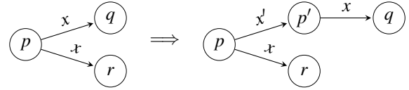
Fig. 1. The 'determinization'; x' and p' are a new event and a new state
