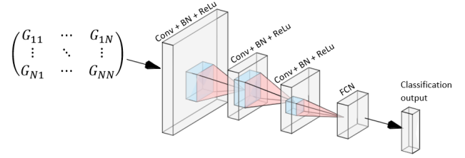
Fig. 2. DL network structure
