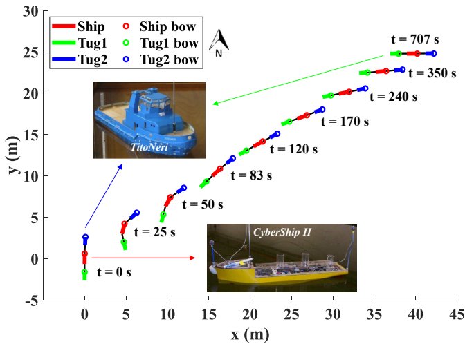
Fig. 7. Simulated towing process.
