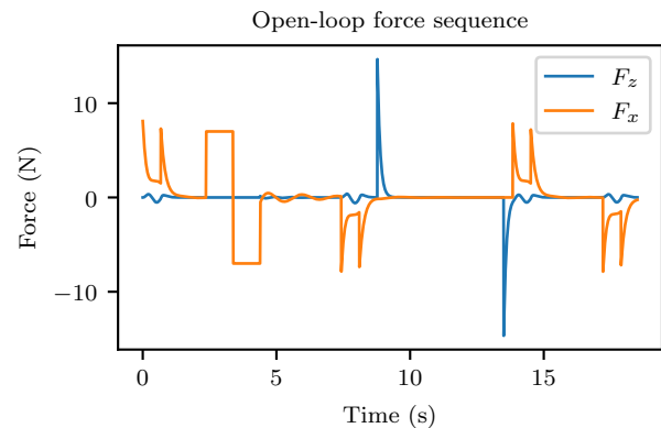
Fig. 13. Input sequence converted to open-loop force commands.
