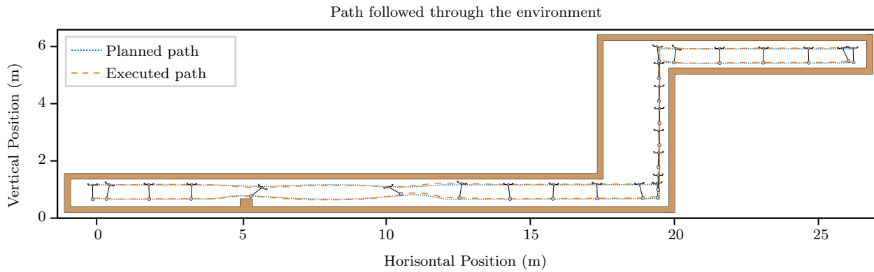
Fig. 11. Path executed by the quadrotor and payload system including actuator dynamics.
