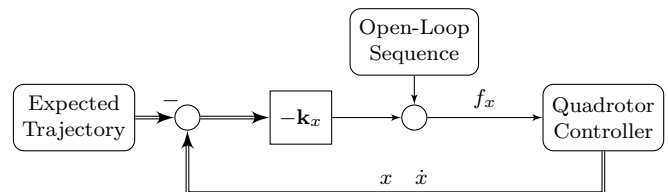
Fig. 10. Control architecture of the horizontal trajectory regulator.
