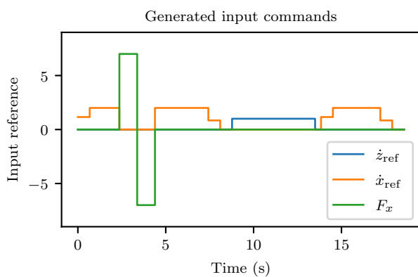
Fig. 12. Input sequence generated by the trajectory planner, consisting of velocity and force commands.
