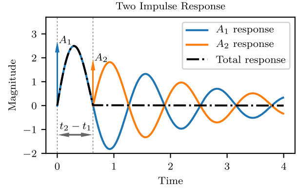
Fig. 4. Two impulse responses resulting in oscillation-free response (Singh and Singhose, 2002). The second impulse, A_2 , is designed to cancel out the response of the first impulse, A_1 .
