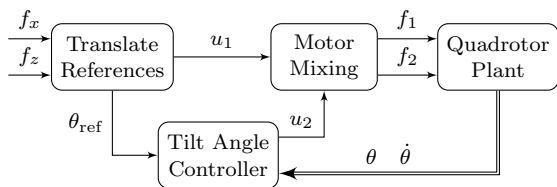
Fig. 9. The flight control system which receives force references to adjust the attitude of the quadrotor UAV.
