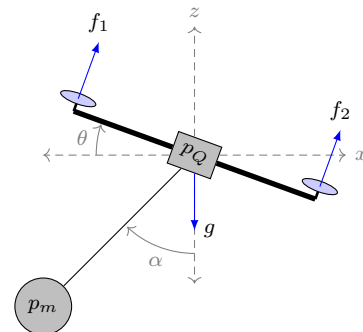
Fig. 3. 2D Model of a quadrotor UAV with a payload suspended through a rigid link.
