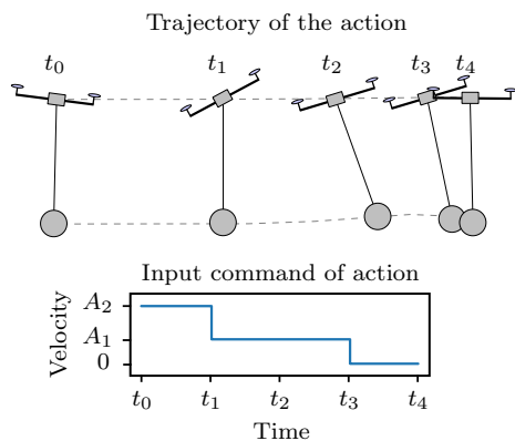
Fig. 7. Action to bring the quadrotor to a standstill.
