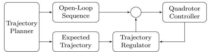
Fig. 2. The system architecture consisting of a trajectory planner and regulator.
