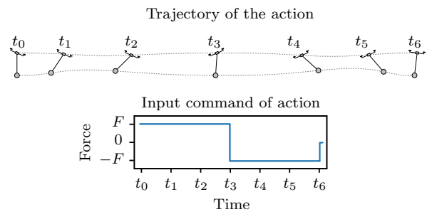
Fig. 8. Action to swing the payload over an obstacle.
