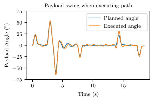
Fig. 14. Payload swing while executing the path.
