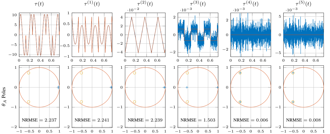
Fig. 2. [Top] Torque signal obtained as in (2) of 3 cams until the 5 th difference. The ideal signal is in orange and the noisy one in blue. [Bottom] Poles of the identified \hat{\theta}_A for the noisy signal (blue), of the applied noise (violet). Notice: the difference signals are processed so to avoid impulses to appear on the cam via-points.
