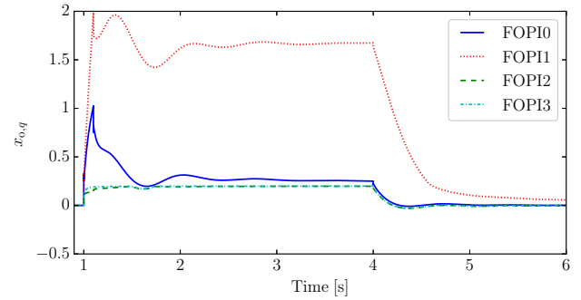
Fig. 7. Response of the integrator state variable of AC voltage controller at outer level.
