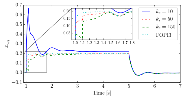
Fig. 8. Response of the integrator state variable of AC voltage controller at outer level for: (i) FOPI2 with different k_s values; (ii) FOPI3.
