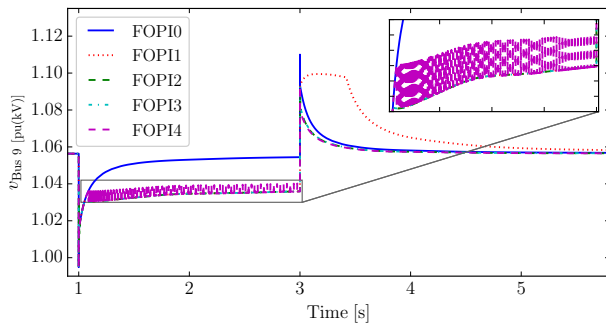
Fig. 9. Response of the voltage at bus 9 considering FOPI0-FOPI4 for the disturbance discussed in Section 4.6.
