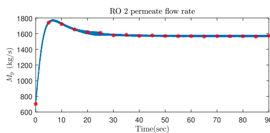
Fig. 9. RO pass 2 permeate flow rate.
