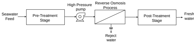
Fig. 1. Diagram of the reverse osmosis plant.
