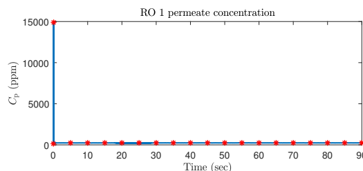
Fig. 8. RO pass 1 permeate concentration.
