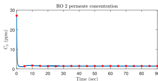
Fig. 10. RO pass 2 permeate concentration.
