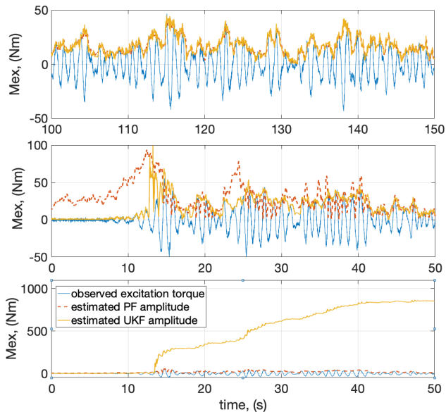
Fig. 4. Comparison of the UKF (yellow line) and PF (red line) observed excitation load amplitudes for the sea state IR1. The measured excitation load (blue line) is used for reference. (Top) fully developed sea state, (Mid) highlights of the initial condition divergence for the PF, and (Bottom) highlights of the initial condition divergence for the UKF.
