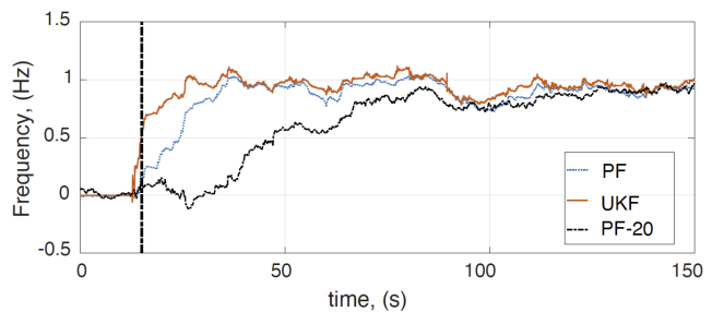
Fig. 5. Observed frequency comparison between UKF (red line), PF (blue line), and under-sampled PF (black line). The ending of the wave ramp-up time is marked with a vertical dotted line.
