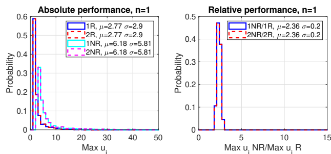
Fig. 5. Probability distributions for n = 1 , maximum control input without and with integral reset (left-hand side), and ratio between maximum control inputs without and with integral reset (right-hand side).
