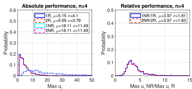
Fig. 8. Probability distributions for n = 4 , maximum control input without and with integral reset (left-hand side), and ratio between maximum control inputs without and with integral reset (right-hand side).
