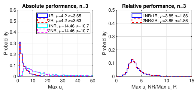
Fig. 7. Probability distributions for n = 3 , maximum control input without and with integral reset (left-hand side), and ratio between maximum control inputs without and with integral reset (right-hand side).
