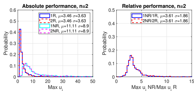
Fig. 6. Probability distributions for n = 2 , maximum control input without and with integral reset (left-hand side), and ratio between maximum control inputs without and with integral reset (right-hand side).
