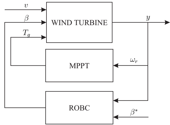
Fig. 1. WT region 2 loads mitigation control
