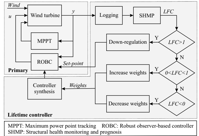
Fig. 5. Proposed adaptive lifetime control scheme
