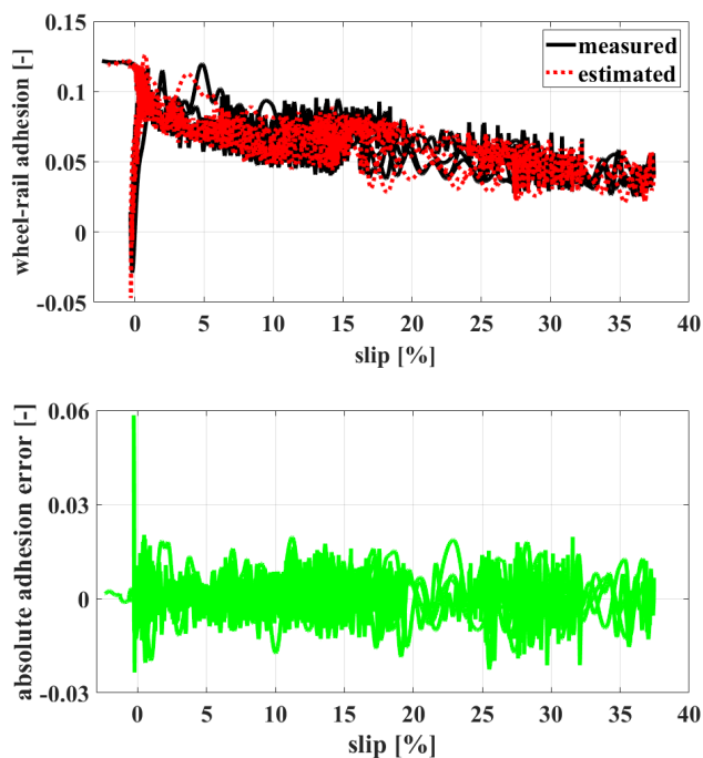
Fig. 6. Top: Comparison of adhesion-over-slip results in a sanding scenario; bottom: Absolute error between estimated and measured adhesion
