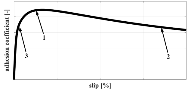
Fig. 3. Qualitative scheme of a typical adhesion over slip characteristic
