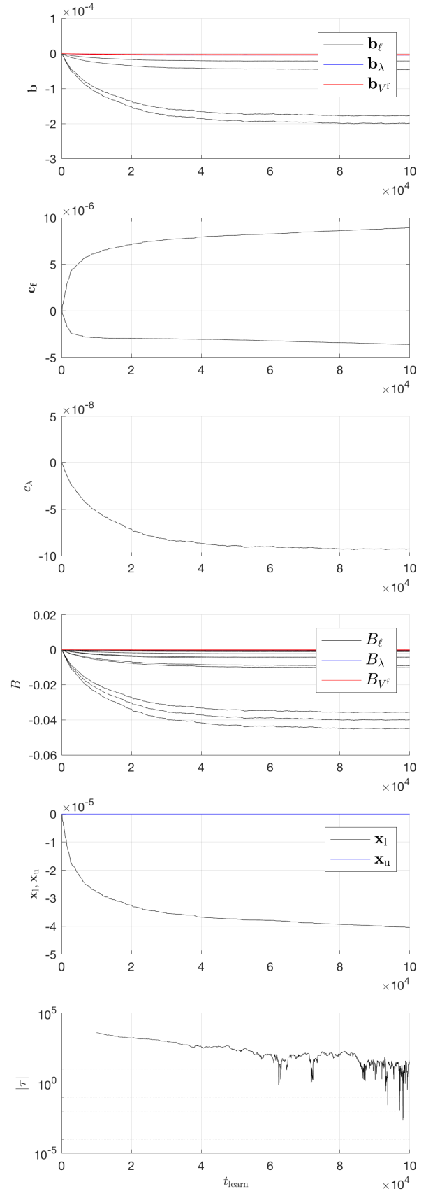
Fig. 1. Evolution of the parameters (increment w.r.t. the initial guess value) and of the TD error (averaged over the preceding 10000 samples).
