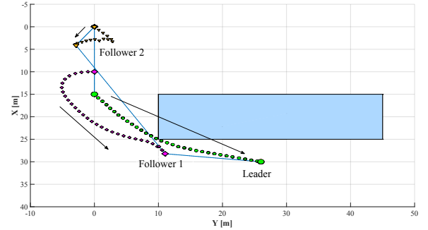
Fig. 6. In this simulation, the leader drone is temporarily prevented from travelling rapidly towards its goal, because its follower would be behind a corner. Once the follower is past such corner, the leader can finally reach its destination.
