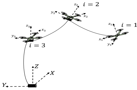
Fig. 1. Model of a considered STEM system with three drones.
