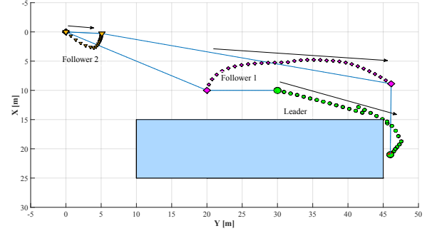
Fig. 6. In this simulation, the leader drone is temporarily prevented from travelling rapidly towards its goal, because its follower would be behind a corner. Once the follower is past such corner, the leader can finally reach its destination.
