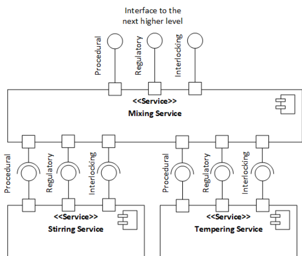
Figure 2: Schematic component model of an orchestrated automation service
