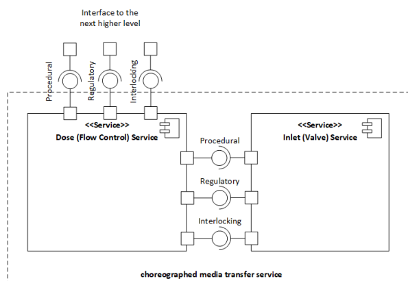
Figure 4: Schematic component model of a choreographed automation service
