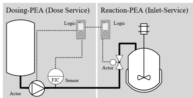
Figure 5: Technological Schema of the media transfer example
