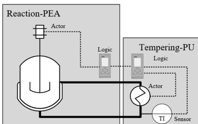
Figure 3: Technological Schema of the mixing example
