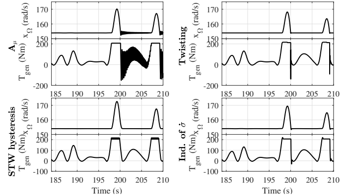
Fig. 6. Rotational speed and control torque for the different algorithms. Top left: A_\mu , top right: TW, bottom left: STW-h, bottom right TW- \hat{\sigma} .
