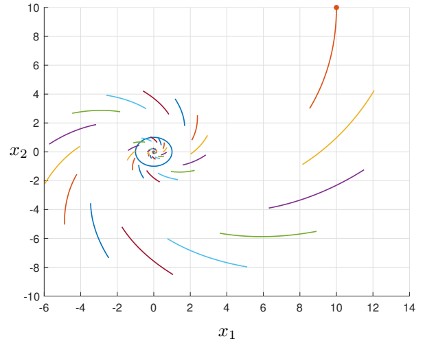
Fig. 2. For \theta > \frac{\ln 2}{2} , trajectories arrive inside a unit circle (unsafe region) for any initial value, e.g., x_0 = (10, 10) .
