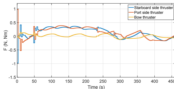
(b) Applied thruster forces.
