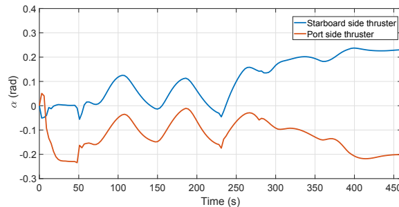
(c) The angle of thrusters.
