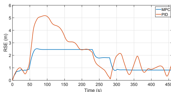
(a) Trajectory tracking RSE: MPC vs. PI.
