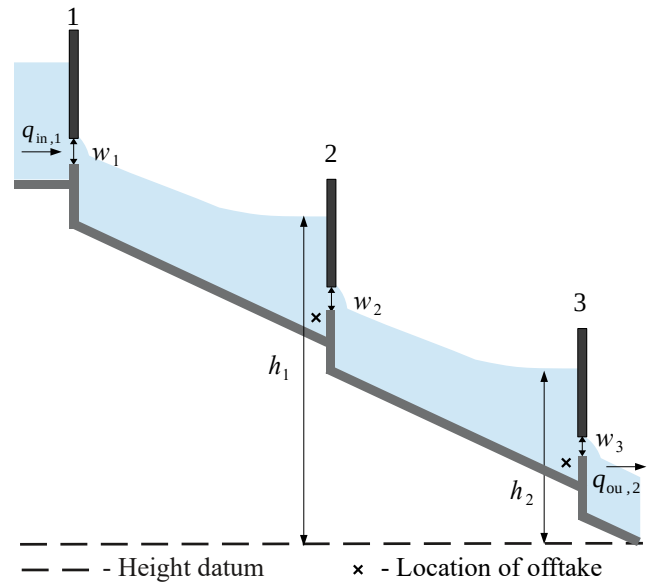
Fig. 1. Start of the primary canal
