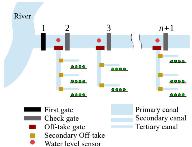
Fig. 1. Start of the primary canal
