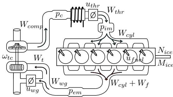
Fig. 1. Schematic of the engine model, where the three states turbocharger rotational speed w_{tc} , intake manifold pressure p_{im} and exhaust manifold pressure p_{em} are displayed. The figure is reproduced with permission from the authors of Ekberg et al. (2018).
