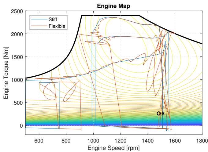
Fig. 8. The engine torque output when performing a fuel optimal acceleration using a stiff (blue) and flexible (red) driveline. The cross \times and circle \circ marks the end points for the stiff and flexible driveline representations. The solid black line is the modeled engine restriction when the maximum torque is set to 2400 Nm, max power to 430 hp and \lambda^{\min} = 1.3 .
