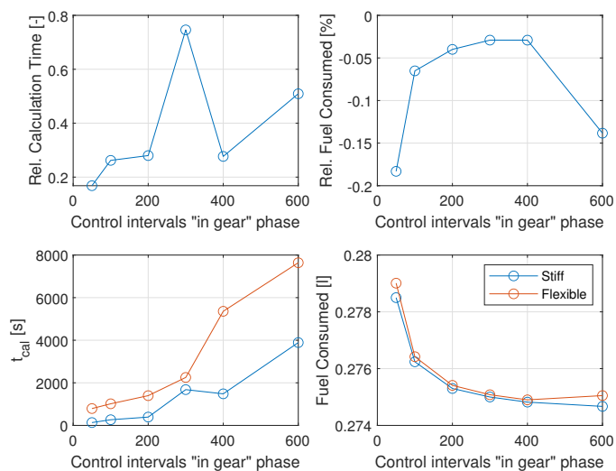
Fig. 12. Calculation time and consumed fuel for stiff and flexible driveline models. The results are simulated with a variable step length ODE solver. The relative measures compare the results from the stiff driveline with the flexible driveline.
