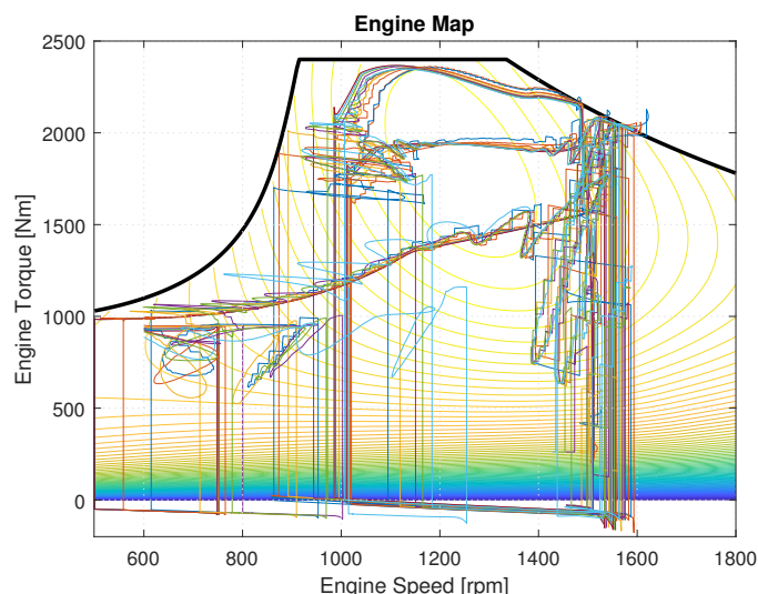
Fig. 11. Results from 12 fuel optimal accelerations using stiff and flexible driveline models. Independent of the driveline model or grid size, all up-shifts are performed between 1500 and 1600 rpm. The engine torque constraint looks to be violated at 1600 rpm, this is due to the results being simulated. When simulating the result, information between the control signal interval end points become visible.
