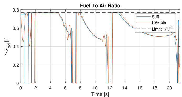
Fig. 10. At the beginning of gear 6, 8, and 10, both the flexible (red) and stiff (blue) driveline are restricted by the fuel to air ratio. There is no way to inject more fuel without producing smoke.
