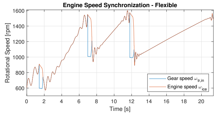
Fig. 9. The engine speed is oscillating during the acceleration. During the gear change the gear speed and engine speed are separated, until the rotational speeds are synchronized by the clutch.
