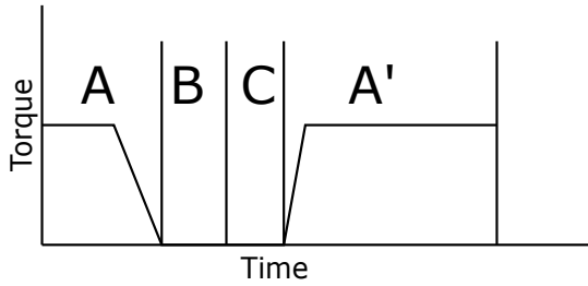
Fig. 5. Example torque demand during a gearshift. The three phases of the gear shift is used as an example to describe how the optimal control models are divided.
