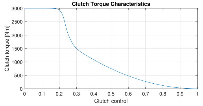
Fig. 2. Model relation between clutch control signal and transferred clutch torque.
