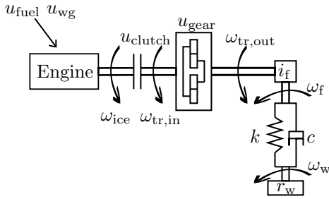
Fig. 3. Schematic of a driveline where the control signals u and rotational speeds \omega are displayed. k and c are the lumped drive shaft stiffness and damping parameters.
