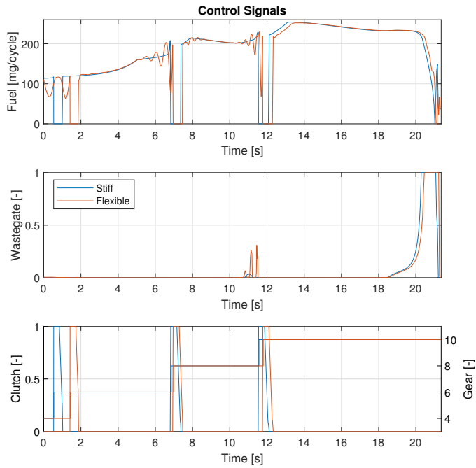
Fig. 7. The wastegate is opening slightly at 11 s and gradually opens at 18 s. The fuel injection profile introduces oscillations in the driveline at the end of each gear.
