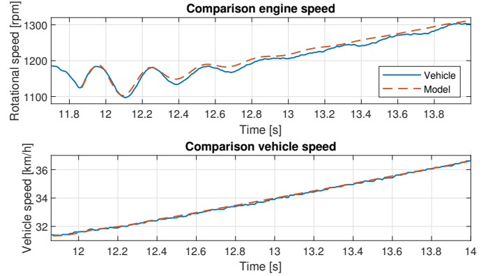
Fig. 4. Validation of the drive shaft stiffness and damping parameters. The wheel speed and engine speed from the acceleration measurement and the vehicle model is compared. The dashed lines are from the model, the solid lines are measurements from the truck.
