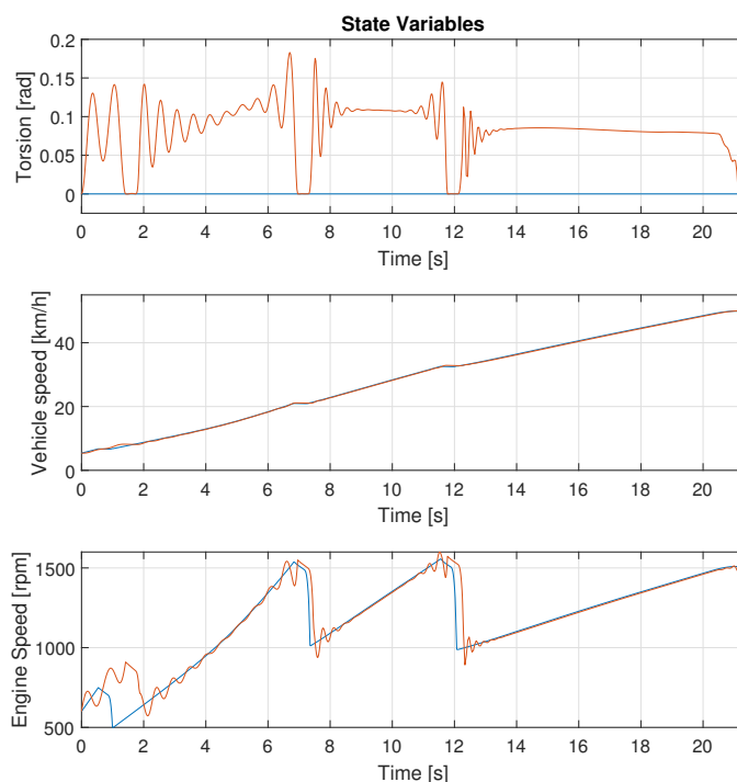
Fig. 6. The acceleration with stiff driveshaft is 0.11 s faster than the flexible, the first gear shift is performed at slightly different engine speeds.
