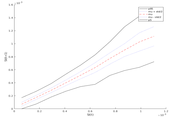
Fig. 8. Mean (red dashed line), standard deviation (two dotted blue lines), and the 5% and 95% percentile values (enveloping black solid lines) of the SI(t + 1) in function of SI(t) in the training data set.
