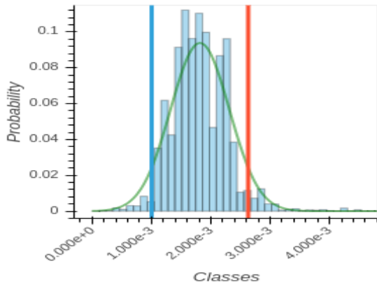
Fig. 5. Output of the CDN network prediction for a given SI(t) value. The fitted Gaussian distribution (green) and the 5% and 95% percentile values (blue and red bars) are also shown.
