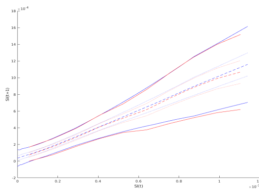
Fig. 12. Comparison of the output of the CDN network prediction with the MDN prediction in function of input SI(t) values. Mean values (middle dashed line), standard deviations (two dotted lines around the mean), and the 5% and 95% percentile values (enveloping solid lines); red: CDN network prediction; blue: MDN prediction.
