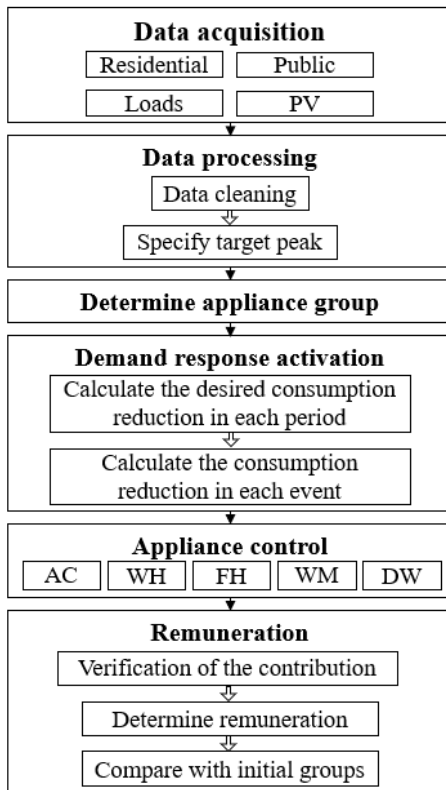
Fig. 1. Proposed Methodology.
